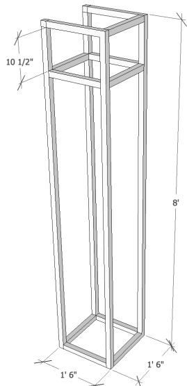
CENTER TOWER ISOMETRIC VIEW
